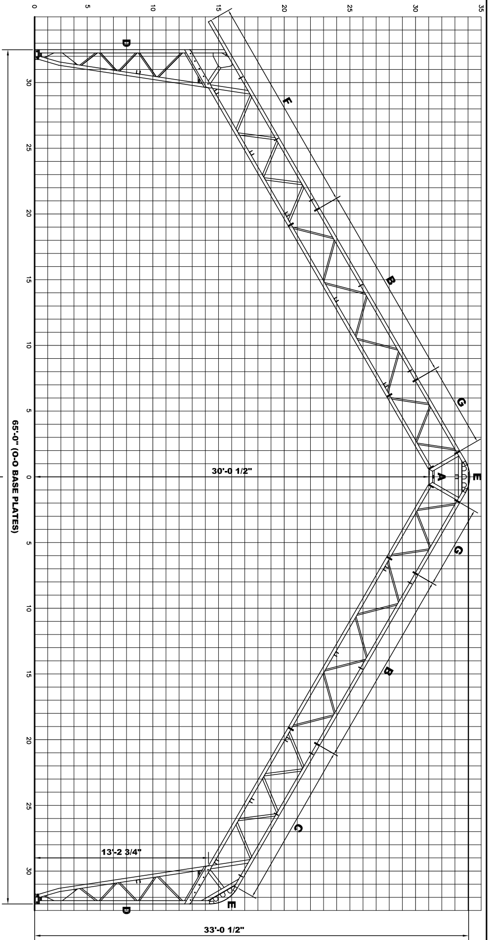
EAVE STRUCTURE (FABRIC - EAVE TO EAVE / PEAK TO EAVE)
